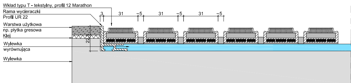
UNIMAT 12 T_M + UR 22
