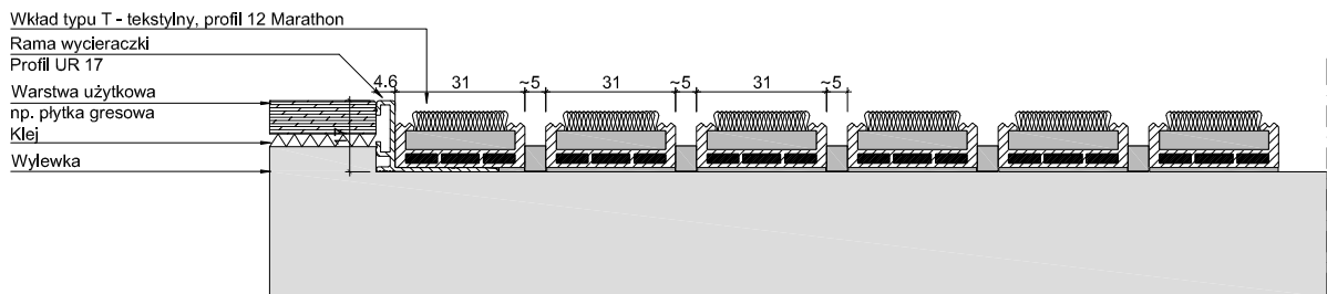
UNIMAT 12 T_M + UR 17
