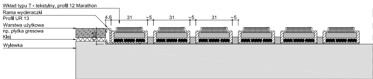
UNIMAT 12 T_M + UR 13
